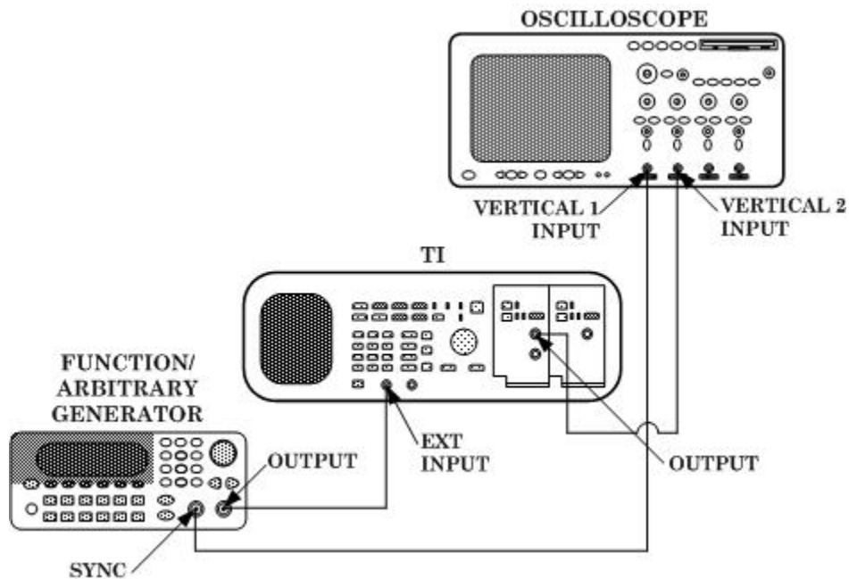
Figure 4. Trigger level and polarity.
